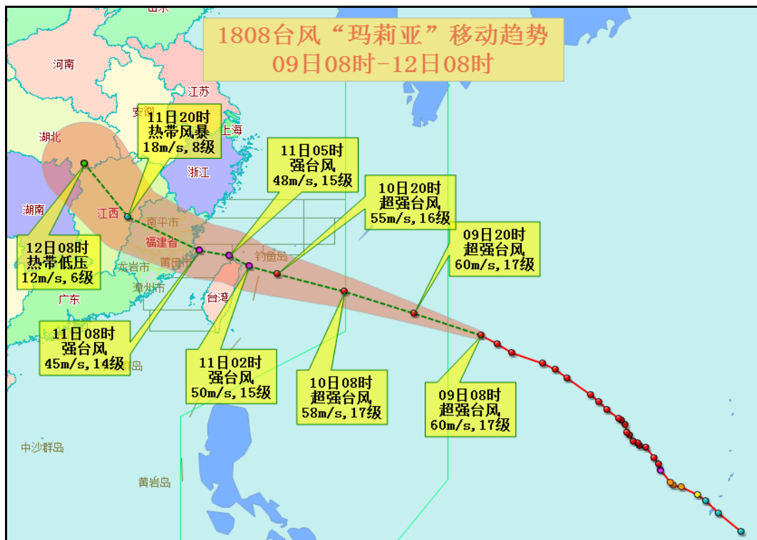
附图：台风“玛莉亚”路径预报
